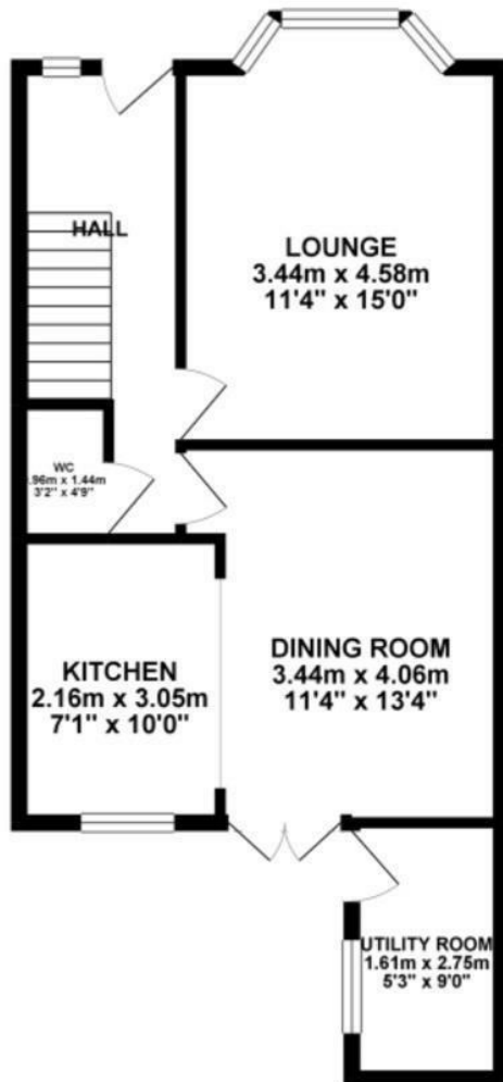
GROUND FLOOR 47.40 sq. m. ( 510.25 sq. ft. )
